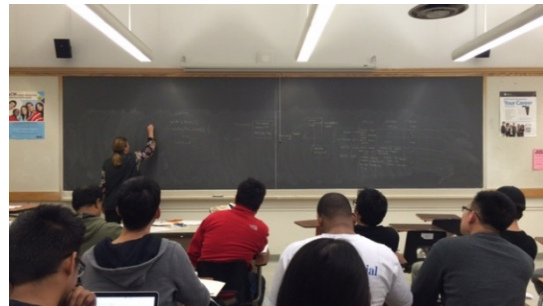
Photo2: Distributed Computing
